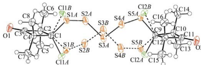
Figure 1 View of the molecule of (IV) after refinement of the initial disordered and inadequate model by standard procedures. The atom labelling scheme and both of the disordered conformations are shown and the view does not reveal any obvious disquieting features. Displacement ellipsoids are drawn at the 50% probability level. H atoms are represented by circles of arbitrary radii.
